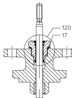
I. EPDM-sealing
