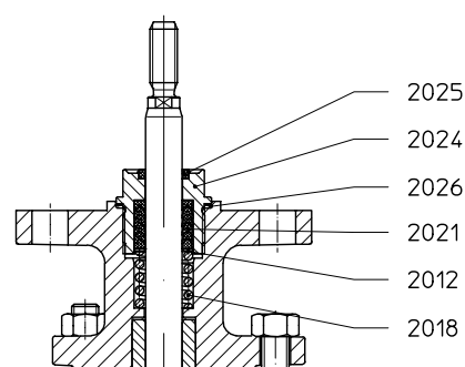
III. Stainless steel-bellows with V-ring unit
