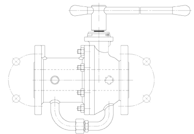
Heating Jacket and special Hand Lever
