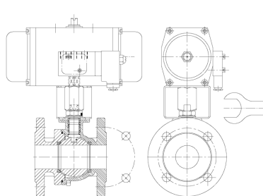
Ball Valve with pneumatic Actuator, Solenoid Valve and Manual Emergency Operation
