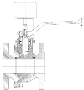
Ball Valve with Limit Switch Box
