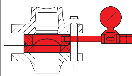
Rupture disc
