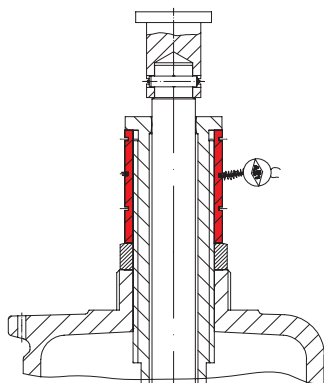
Lock bushing
