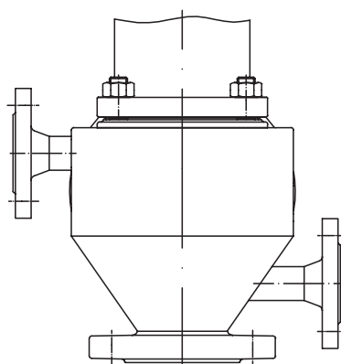
Heating jacket
